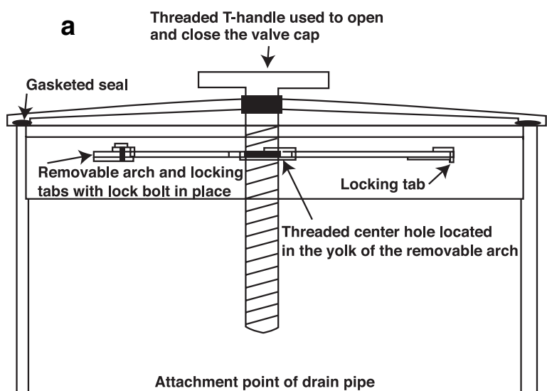
Figure 3. Cross-sectional side (a) and overhead (b) view of an alfalfa valve with a removable arch.
