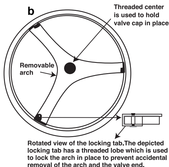
Figure 3. Cross-sectional side (a) and overhead (b) view of an alfalfa valve with a removable arch.
